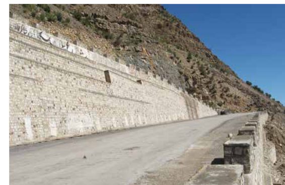
既存道路の石積み擁壁（建設前）／Masonry retaining walls for the existing road (before the construction work)
