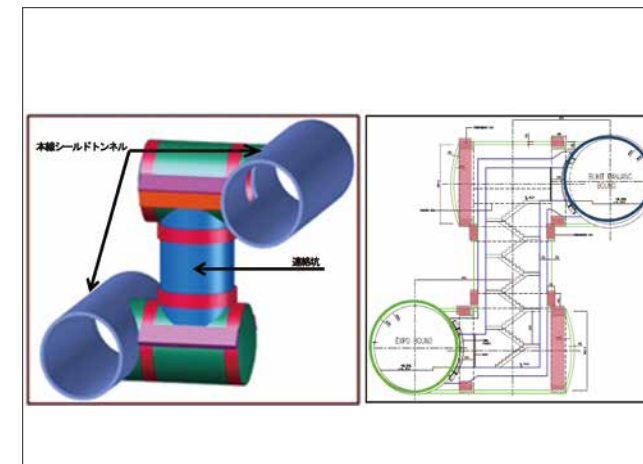
上下線間にある連絡坑を、地上からの立坑から非開削のNATM工法に変更し、 周辺環境への影響を低減／ For connecting cross passage between inbound and outbound lines, method for constructing vertical shafts from ground level was altered to a non-open-cut NATM method to reduce impact on the surrounding environment.
