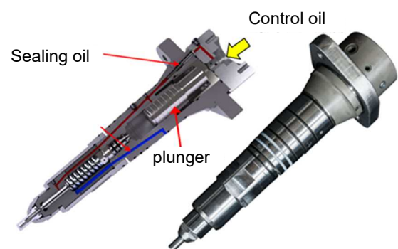
Figure Appendix 3.2-3: Ammonia Fuel Injection Valve (Fuel Booster Injection Valve, FBIV)
