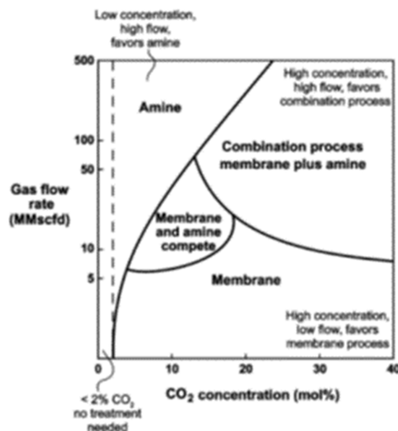
Figure Appendix 3.3-4: \text{CO}_2 Separation Capacity under High-pressure Conditions
