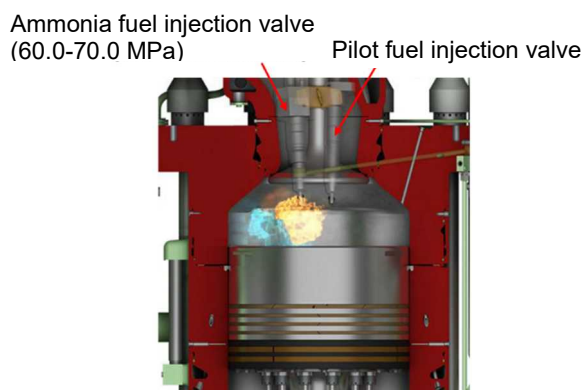
Figure Appendix 3.2-2: Ammonia-powered Engine
