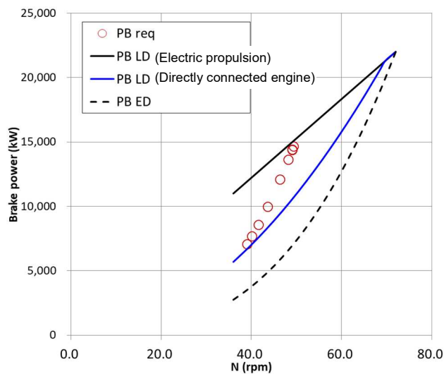
Figure Appendix 3.4-4: Load Diagram and Results of the Assessment of Minimum Propulsion Power
