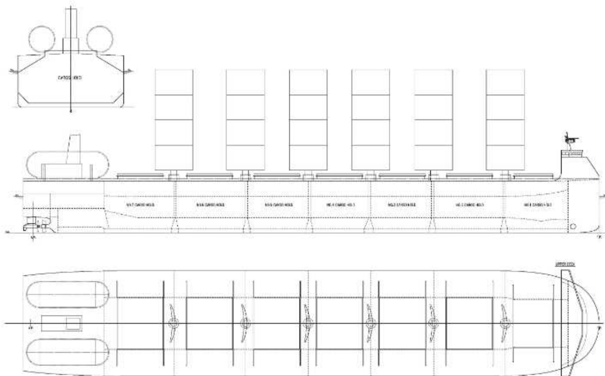
Figure 4.4.4-1: General Arrangement of the Super-efficient LNG-Fueled Bulk Carrier
