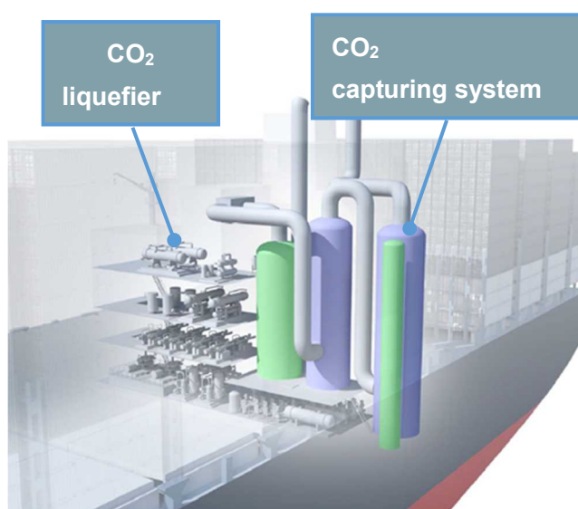
Figure Appendix 3.3-6: 20,000 TEU Container Ship's CO 2 Capturing System
