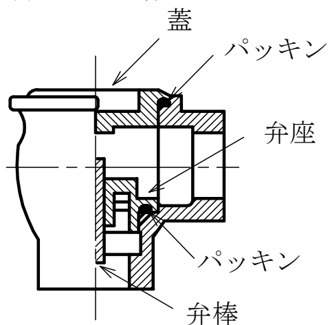
(a) 注油逆止弁
