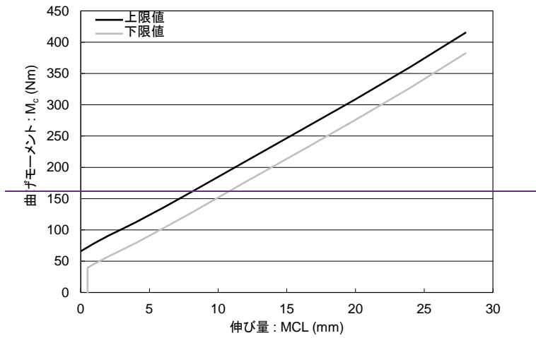
(a) for MCL
