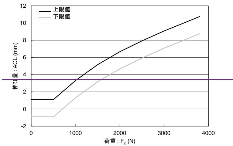
(b) for ACL
