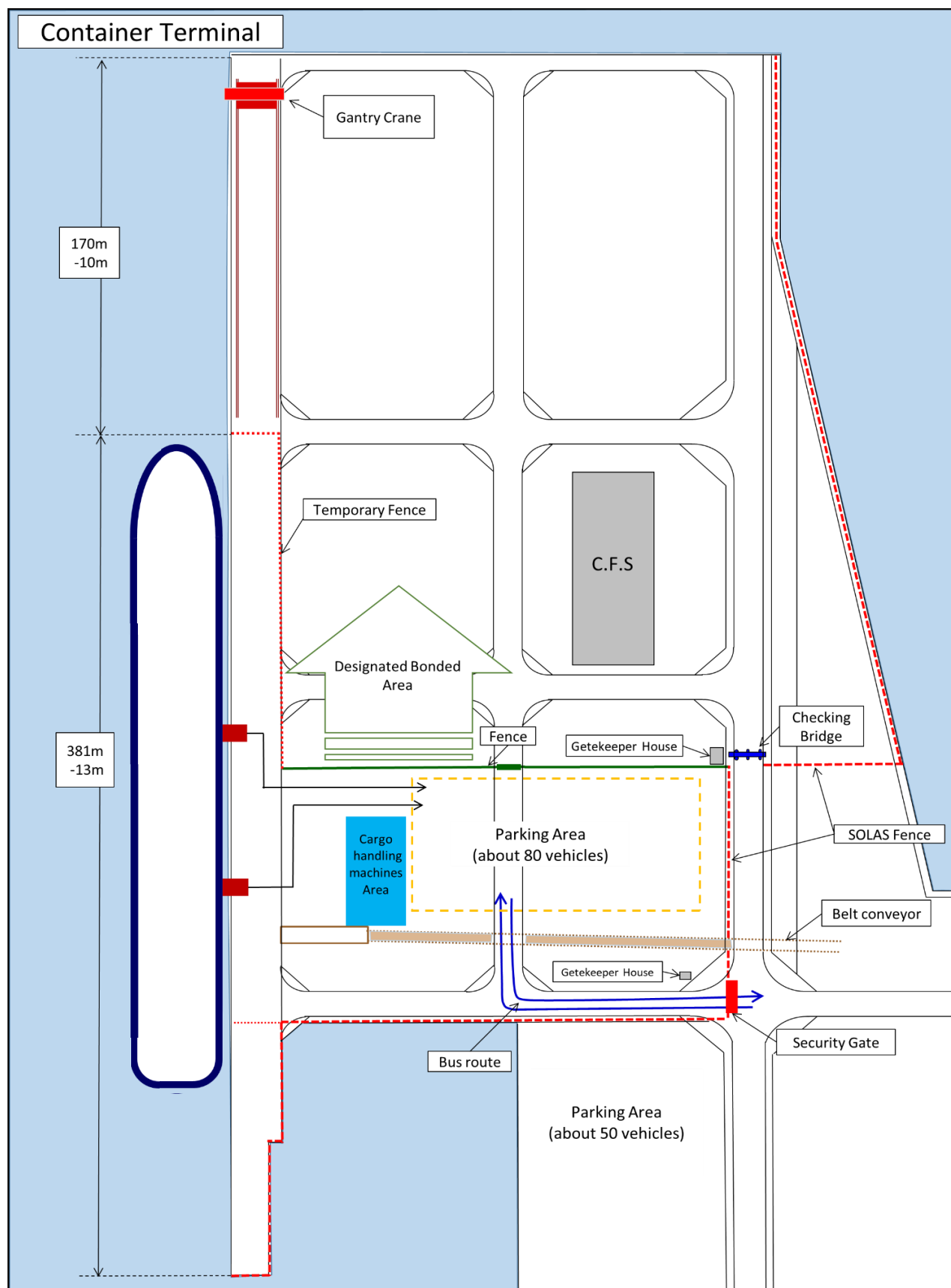
Figure of the terminal placement and passenger line of flow ターミナル配置図と受入動線
