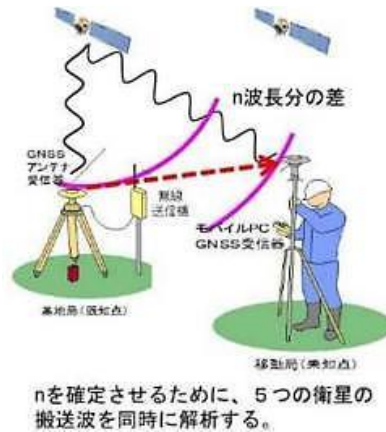
図- 1.1 RTK-GNSS
