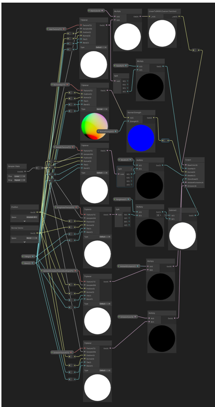
図3-1-15 PlateauTriplanarSubGraphの実装
