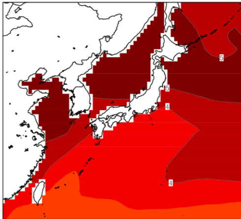
Sea Surface Temperature [Summer] 4K MI - HPB
