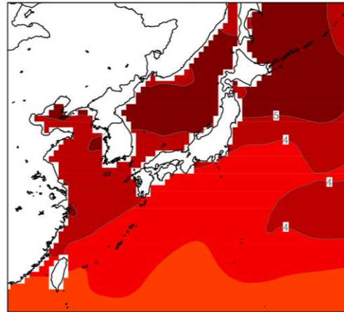
Sea Surface Temperature [Summer] 4K GF - HPB
