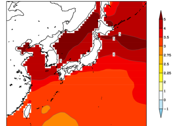
Sea Surface Temperature [Summer] 4K MR - HPB
