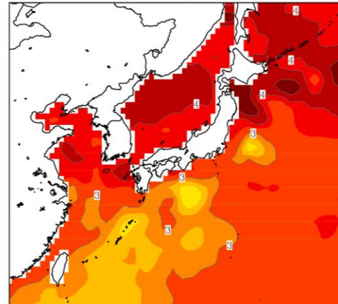
Sea Surface Temperature [Summer] 4K MP - HPB
