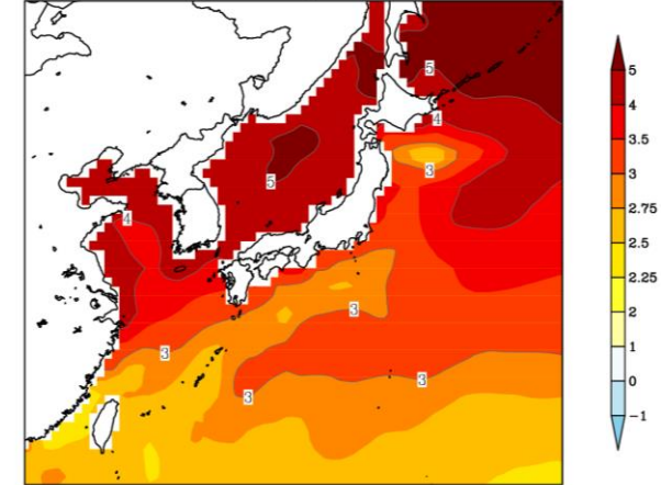
Sea Surface Temperature [Summer] 4K HA - HPB
