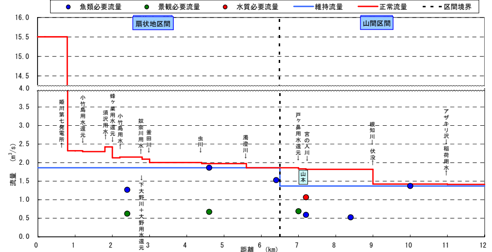
[水収支縦断面図（非かんがい期：9/11～4/15）]
