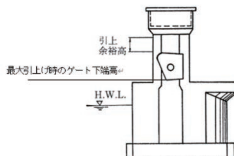
図7-24 門柱
