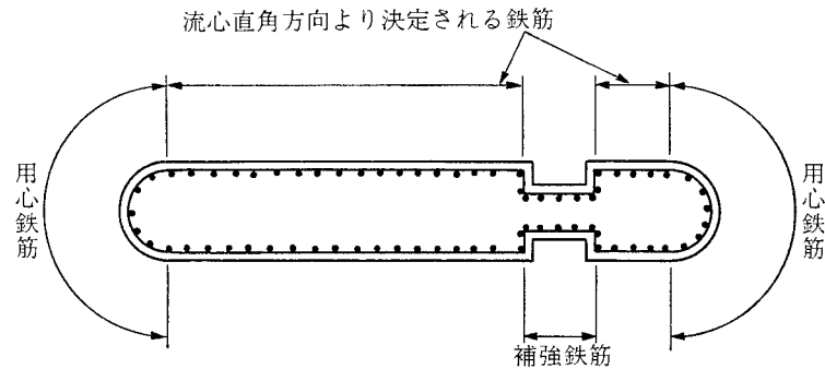
図7-20 堰柱の配筋
