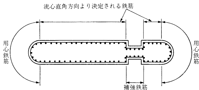
図9-10 堰柱の配筋
