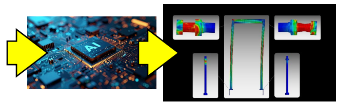
▲The stress distribution of the structure can be visualized based on the bolt axial force
